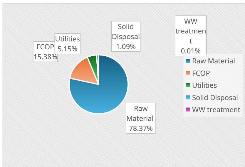
Figure 11: Operating Cost Breakdown (%)
