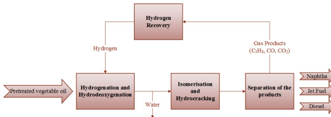
Figure 6: HEFA Block Flow Diagram
