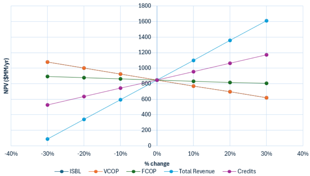
Figure 16: MACRS-5 year sensitivity analysis
