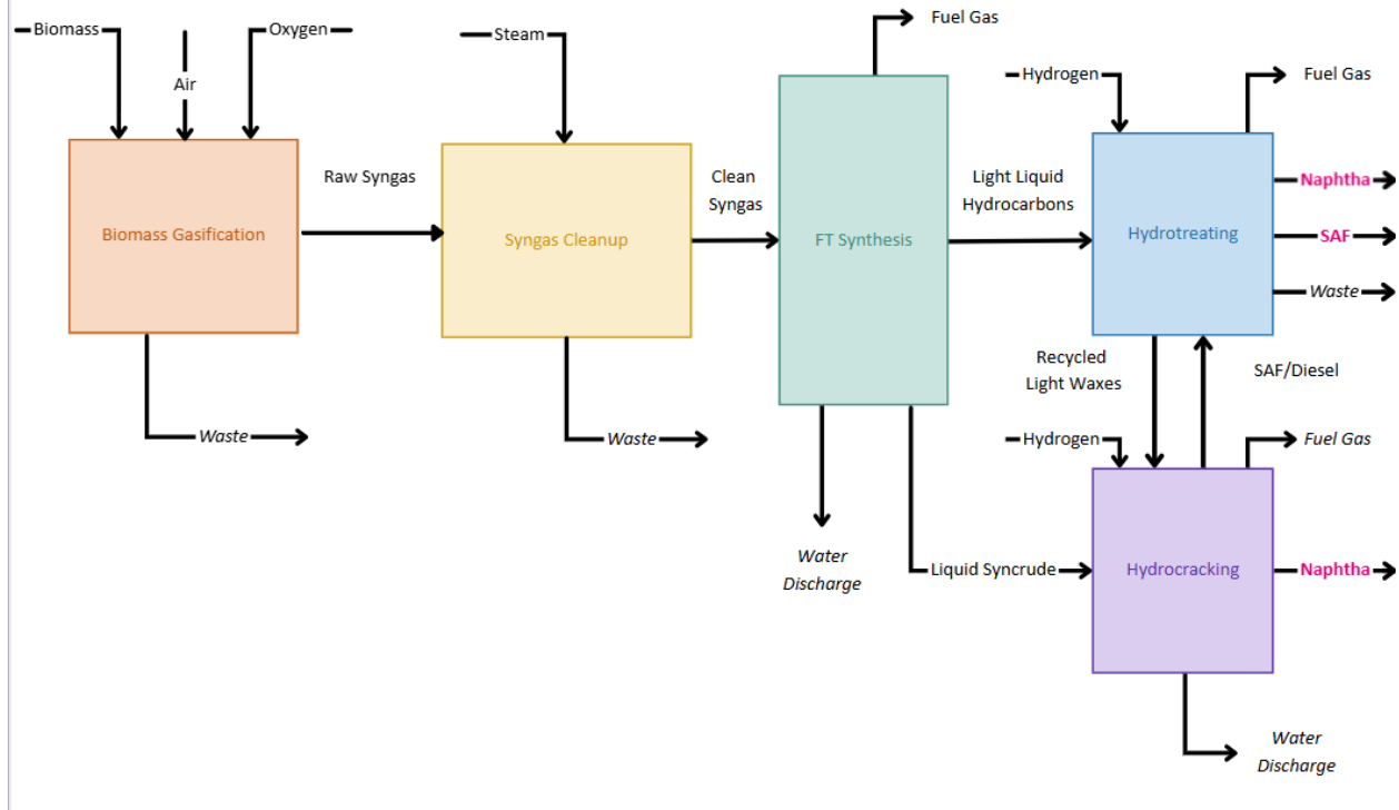
Figure 18: Final Block Flow Diagram
