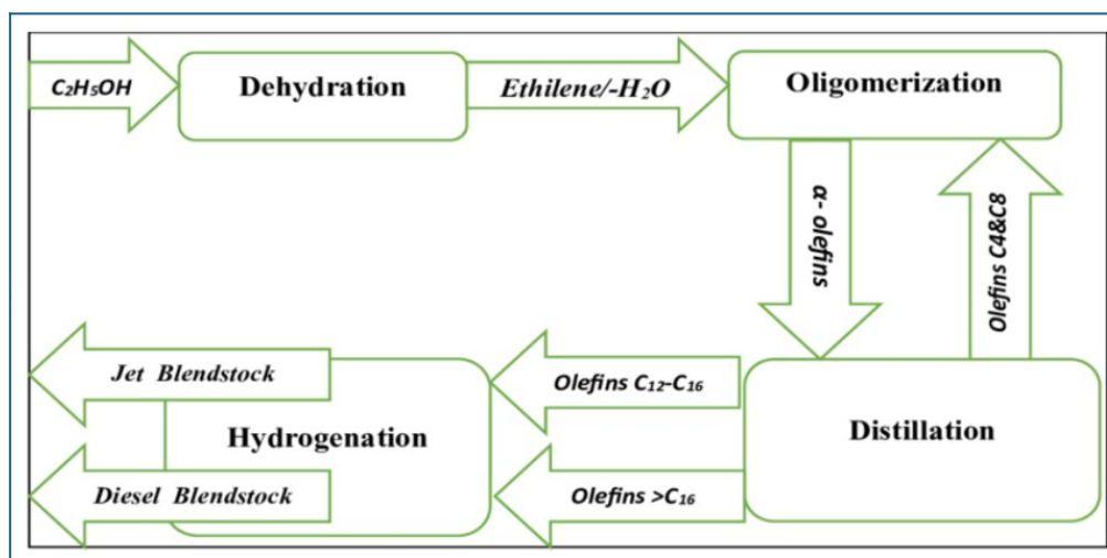
Figure 7: ATJ Block Flow Diagram
