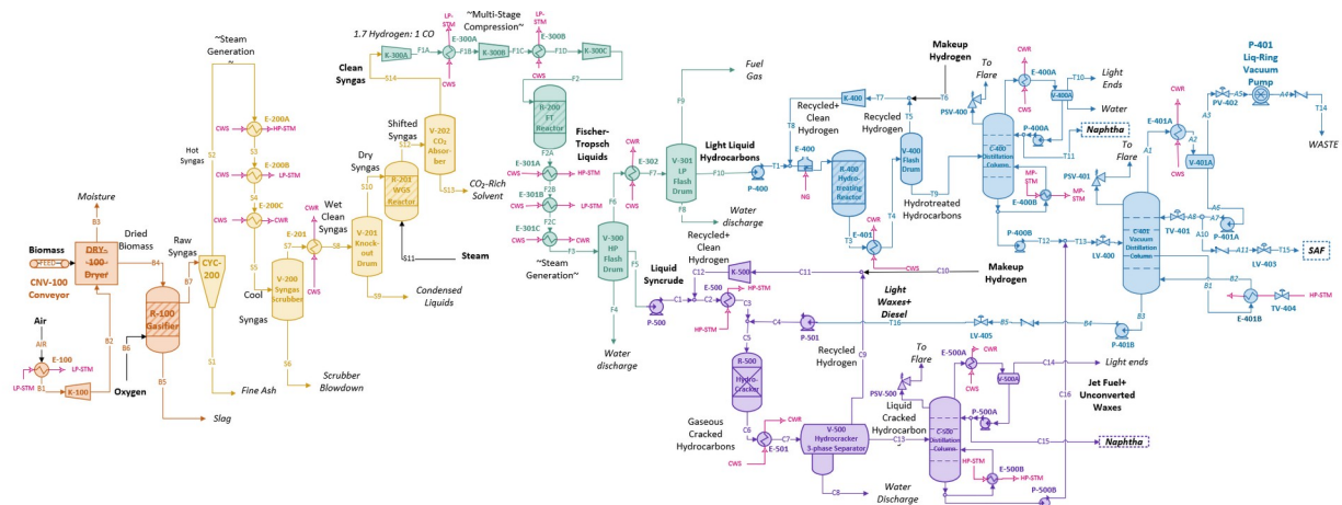
Figure 19: Final Process Flow Diagram
