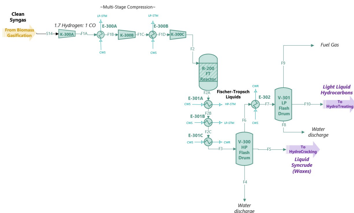
Figure 3: Fisher-Tropsch Synthesis Process Flow Diagram
